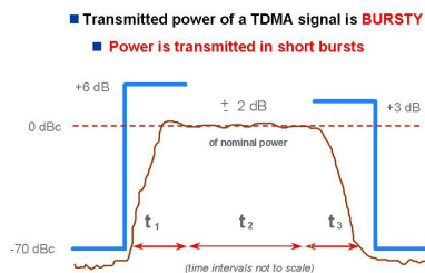
Figure 2 - TETRA Power Profile Mask
