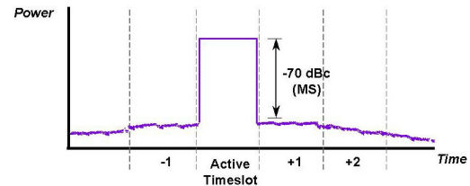
Figure 3 - Performance Requirements of a TDMA Systems
