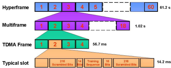
Figure 1 - Air Interface - TDMA illustrated
